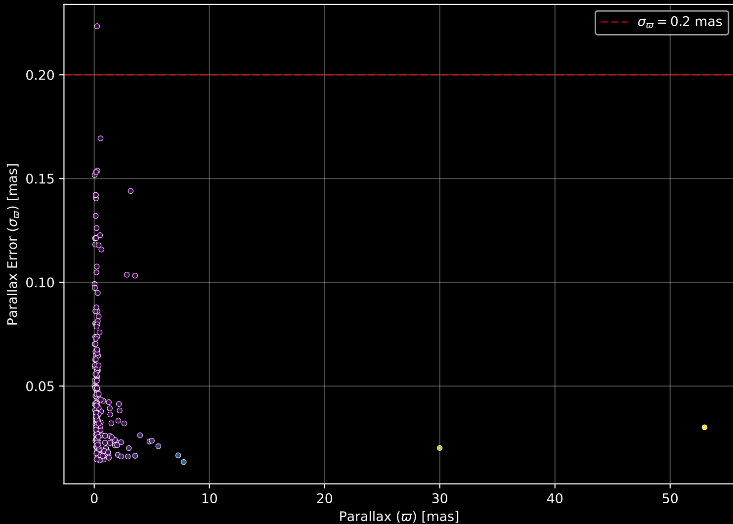
APOGEE DR17 Field: [038+04] Parallax Quality (n= 193)
