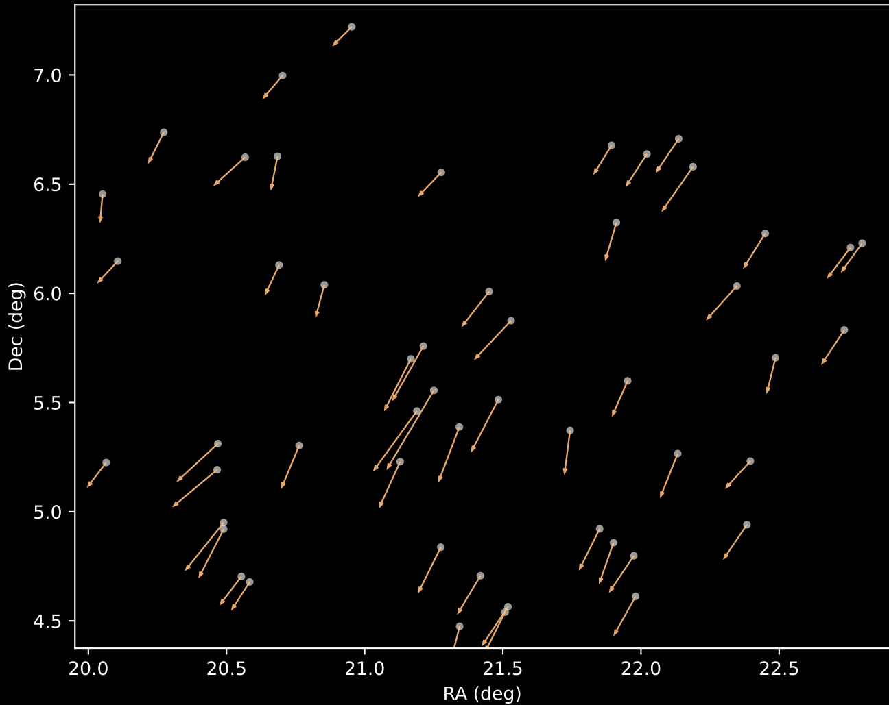
APOGEE DR17 Cluster 3 Proper Motion Vectors (n=52)
