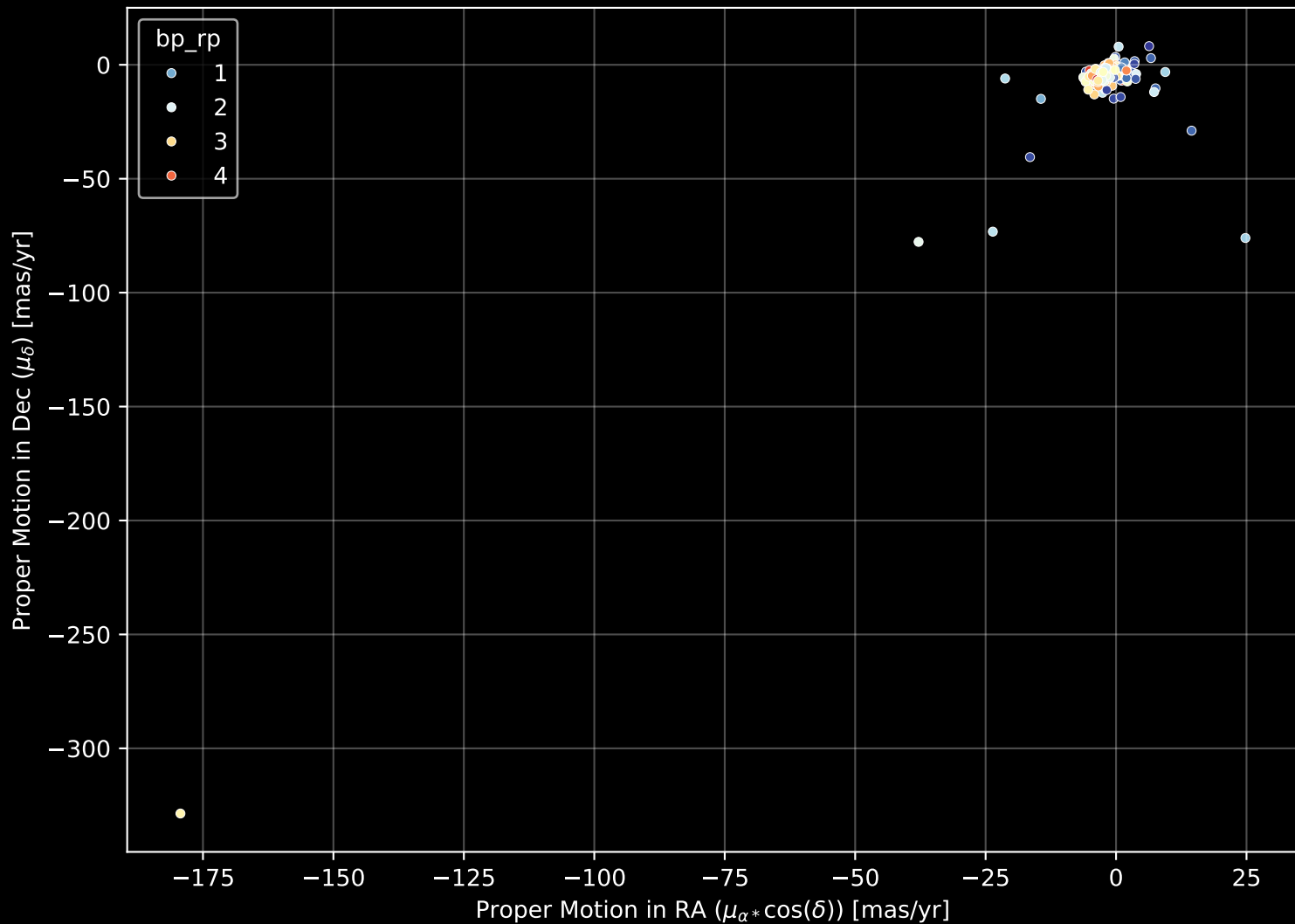
APOGEE DR17 Field: [038+04] Proper Motion Diagram (n= 193)
