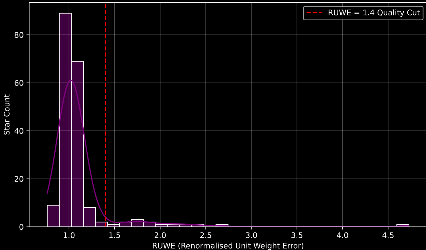
GAPOGEE DR17 Field [038+04] RUWE Distribution (n= 191)
