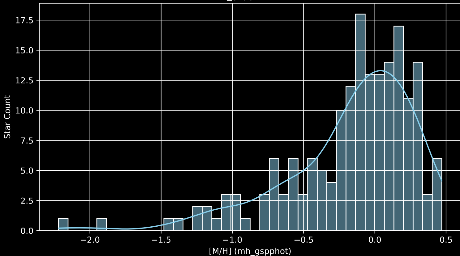
APOGEE DR17 Field: [038+04 [M/H] (mh_gspphot) (n= 183)
