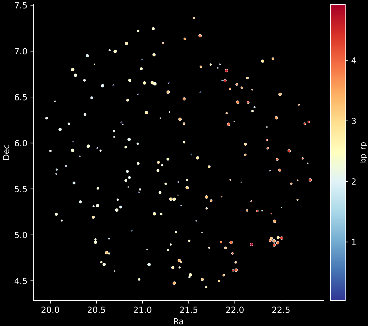
APOGEE DR17 Field: [038+04] Stars: 193
